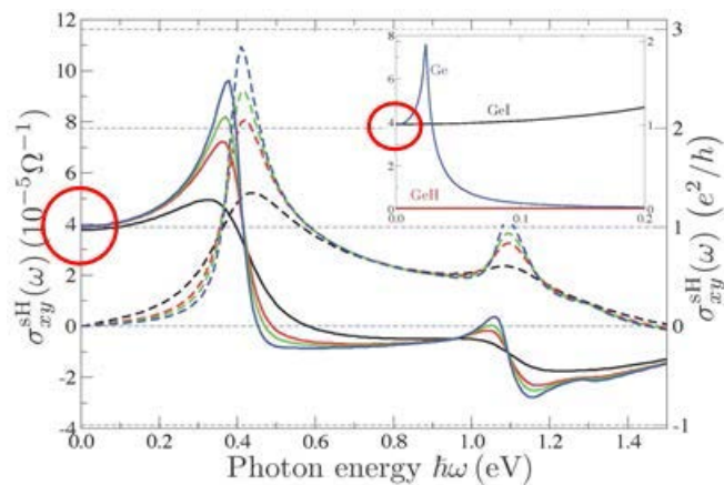
Fig. 1: Real (solid) and imaginary (dashed) part of spin Hall conductivity for Ge, GeI and GeH.
